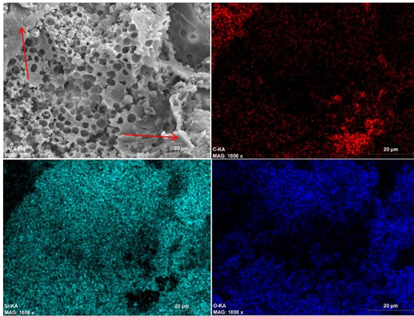
Figure 28: EDS elemental maps of sample L-17-DK-04 of an area covered by spherical algae cells. There are two carbon-rich areas (red arrows) made of EPS. The area covered by the algae cells is silica-rich, suggesting that these are siliceous algae.
