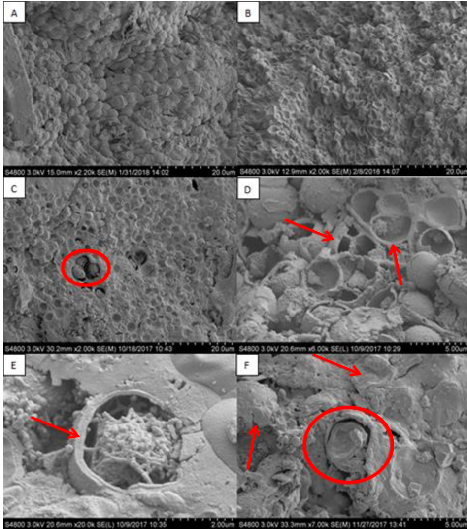
Figure 24 A-F: Panels A and B are from sample L-17-DK-27 and panels C-F are from L-17-DK-04. (A) A large region covered in sub-spherical algae cells with ropy texture and furrowed surfaces. (B) Another region covered in a colony of algae cells with a different morphology. The algae cells are biconcave and often oval shaped. (C) Large areas are covered by a honeycomb texture where spherical algae cells have fallen off the substrate. The red circle shows an area with three-fold symmetry where algae cells were caught in the middle of cell division. (D) Sub-spherical algae cells with cross section visible, showing three separate cells connected at the center indicating that it was in the middle of cell division. (E) Algae cell with cross section visible showing intercellular material and a two-layered cell wall. The red arrow points at the two distinct cell wall layers. (F) The red circle shows a biconcave shaped algae cell that has been broken open leaving a visible cross section, revealing a distinct cell wall and intercellular material. The red arrows show mounded structures that are likely other algae cells covered in amorphous silica.
