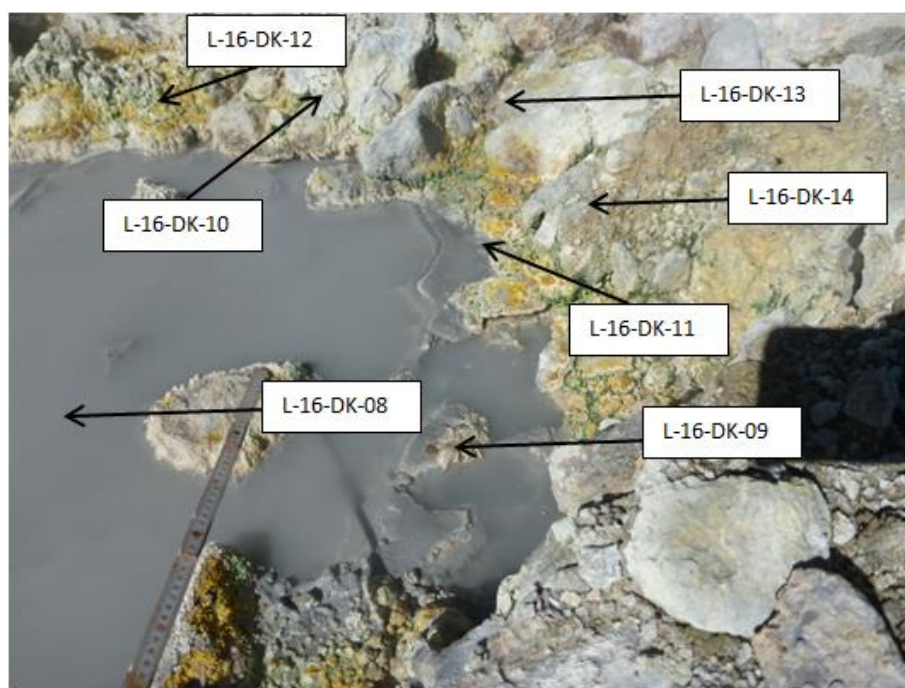
Figure 10: Site 2: In 2016, samples L-16-DK-08 to L-16-DK-14 were collected from around this hot spring and in 2017 samples L-17-DK-07 to L-17-DK-11 were collected. A foldable meter stick is shown for scale
